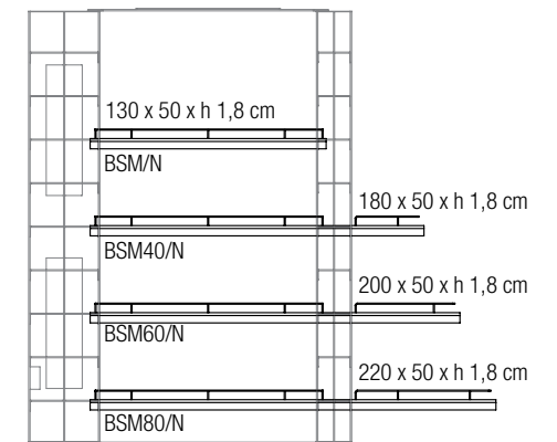
MENSOLE IN PANNELLO PANEL SHELVES
