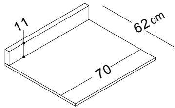
BTOP70 top retro banco spessore 2 cm L70 top for back counter thickness 2cm L70
