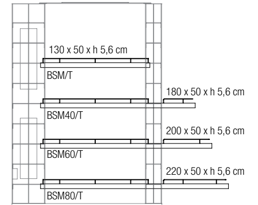
MENSOLE IN TAMBURATO HONEYCOMB SHELVES
