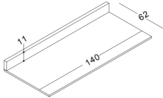
BTOP140 top retro banco spessore 2cm L140 top for back counter thickness 2cm L140
