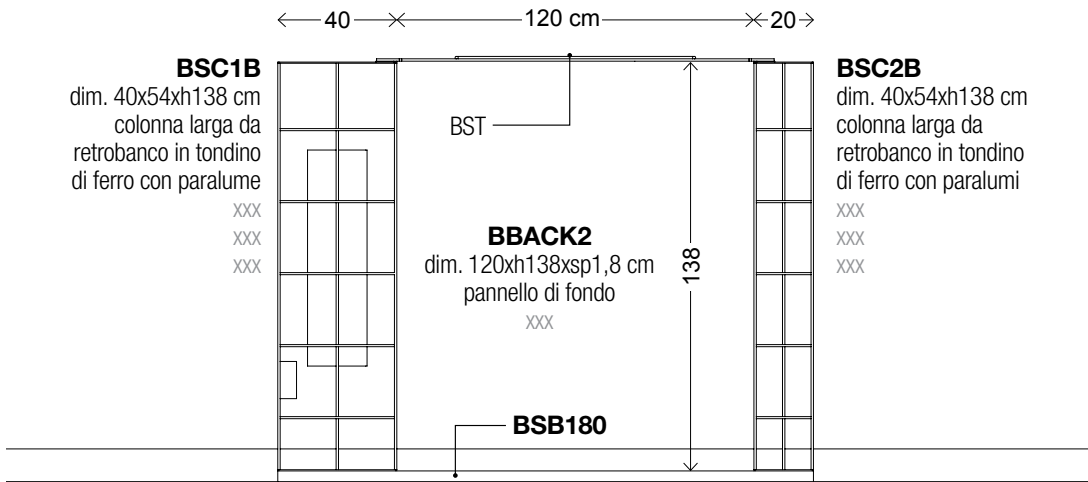
SELF STANDING RETRO BANCO XXX
